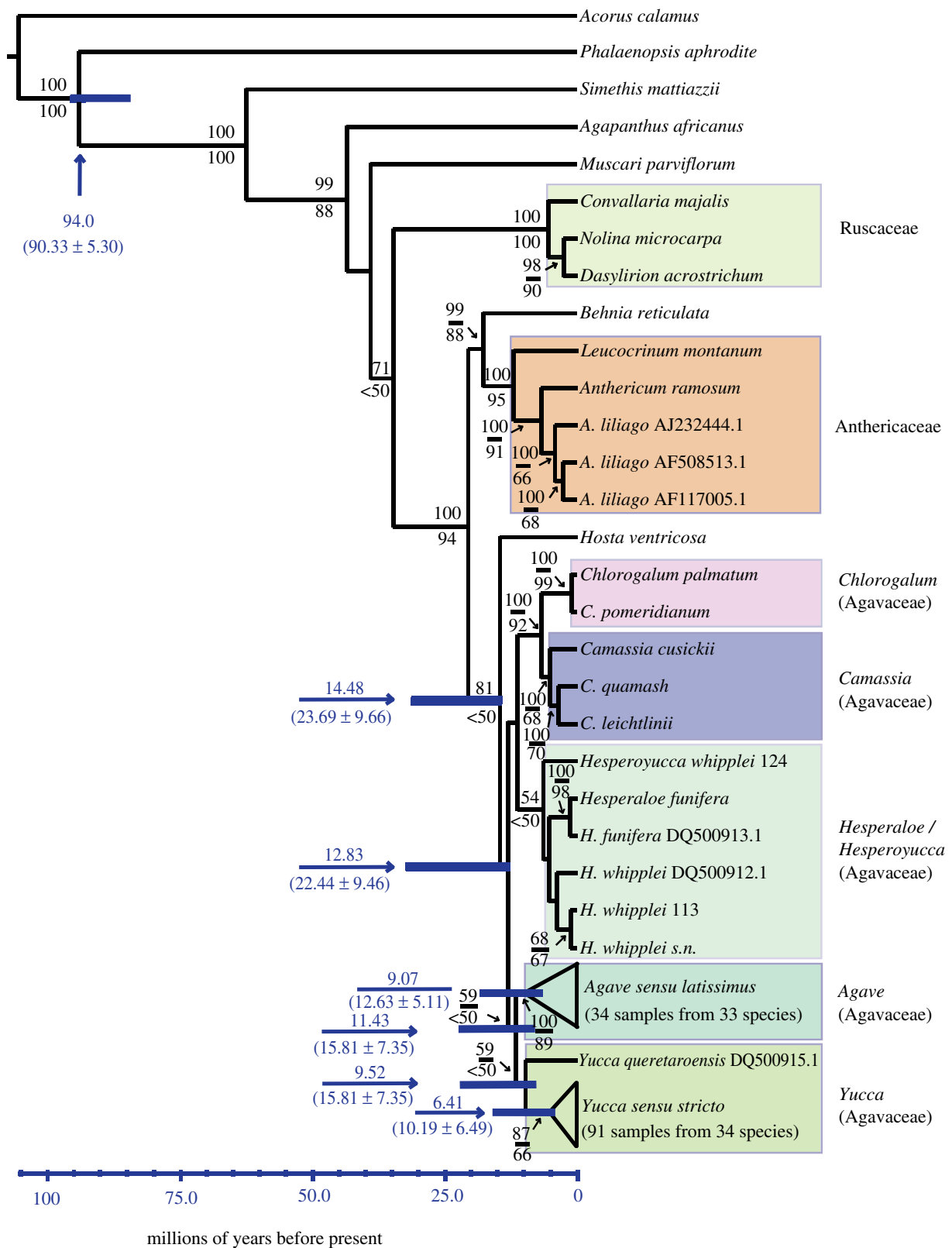
Figure 1. Chronogram of the Agavaceae based on the Bayes consensus tree derived from 153 cpDNA sequences from the trnL gene and the trnL – trnF intergenic spacer. Amborella trichopoda was used to root the topology and was pruned in the r8s analysis. Node labels show Bayesian posterior probabilities (above) and non-parametric bootstrap supports (below). Unlabelled nodes have less than 50% support. Error bars represent the standard deviation of age estimates profiled across post-burn-in trees (below the arrow; values above the arrow represent the node age in Bayes consensus). For the complete consensus tree, see electronic supplementary material.
